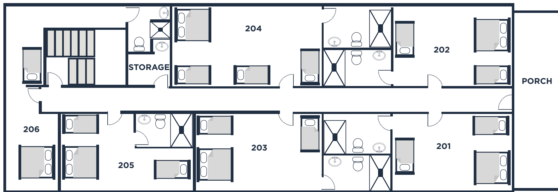
UPPER LEVEL
